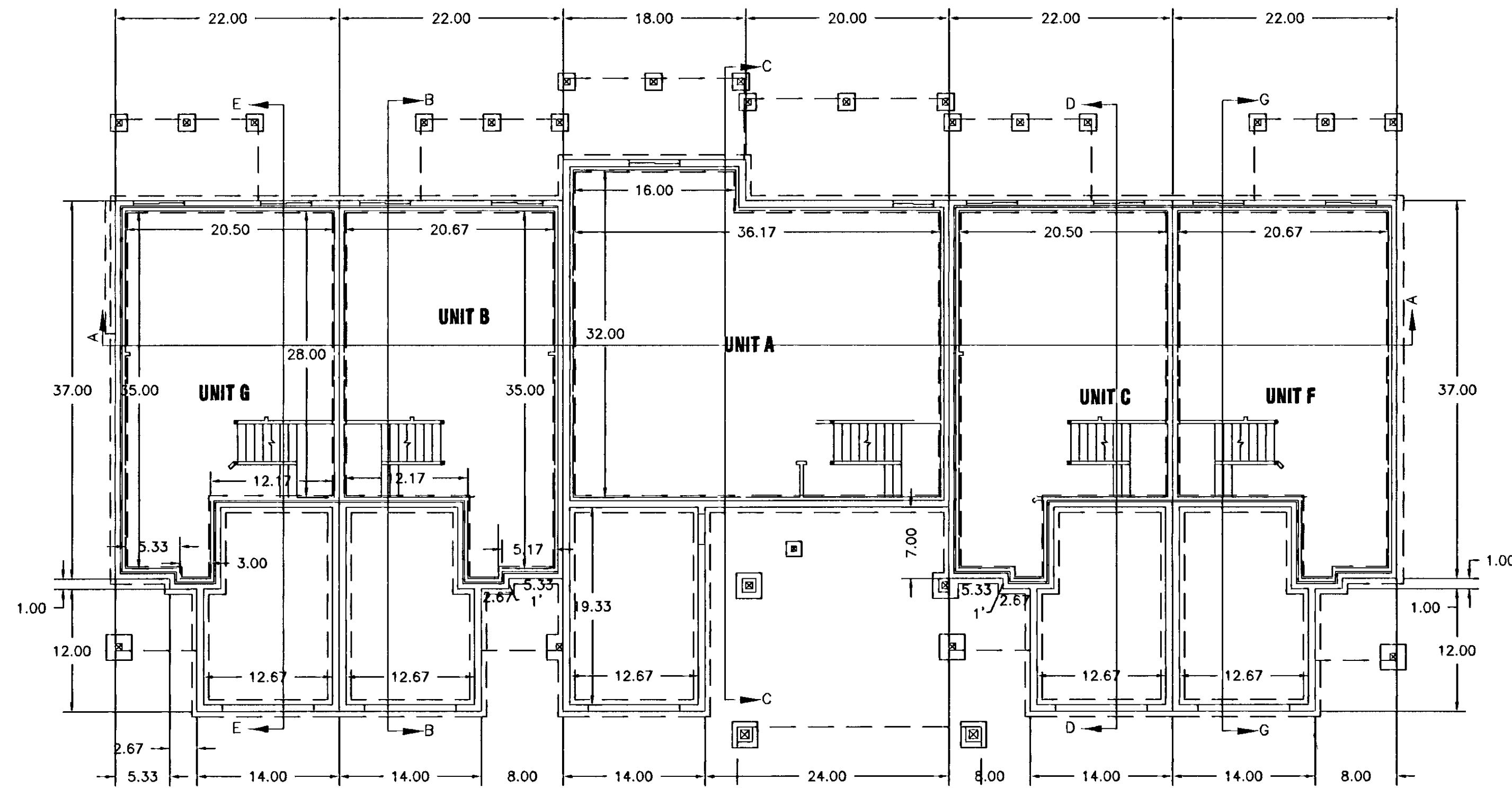
BASEMENT LEVEL SCALE: 1"=10'
