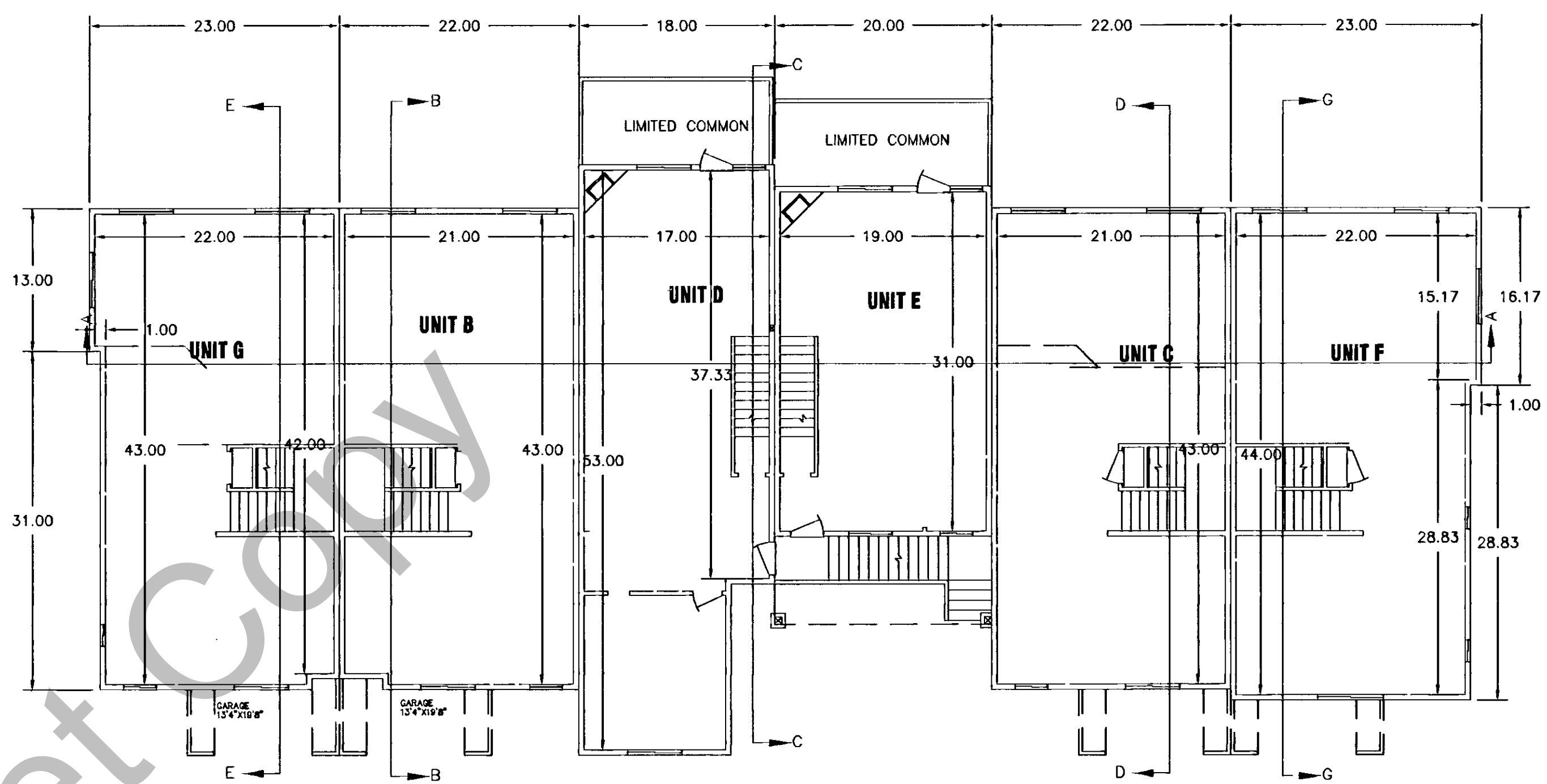
SECOND LEVEL SCALE: 1"=10'
