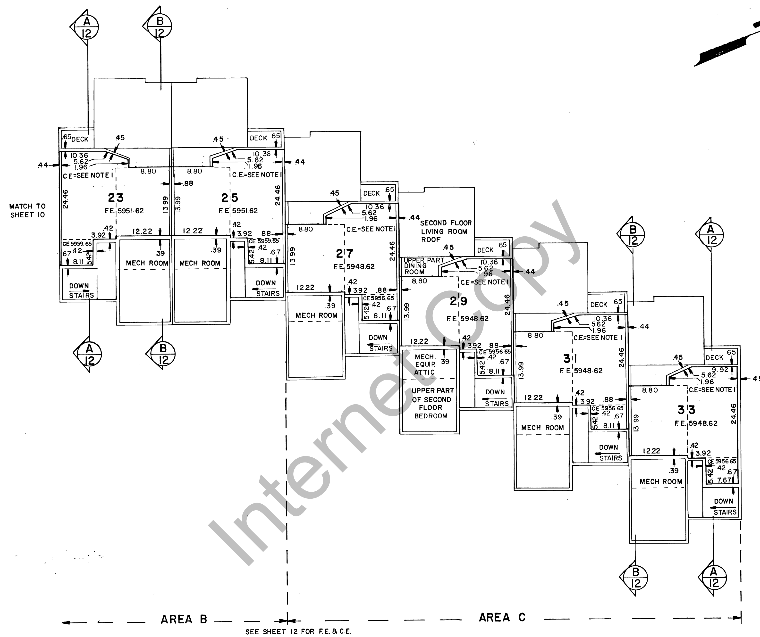
BUILDING B THIRD FLOOR PLAN SCALE: 1" = 10'
