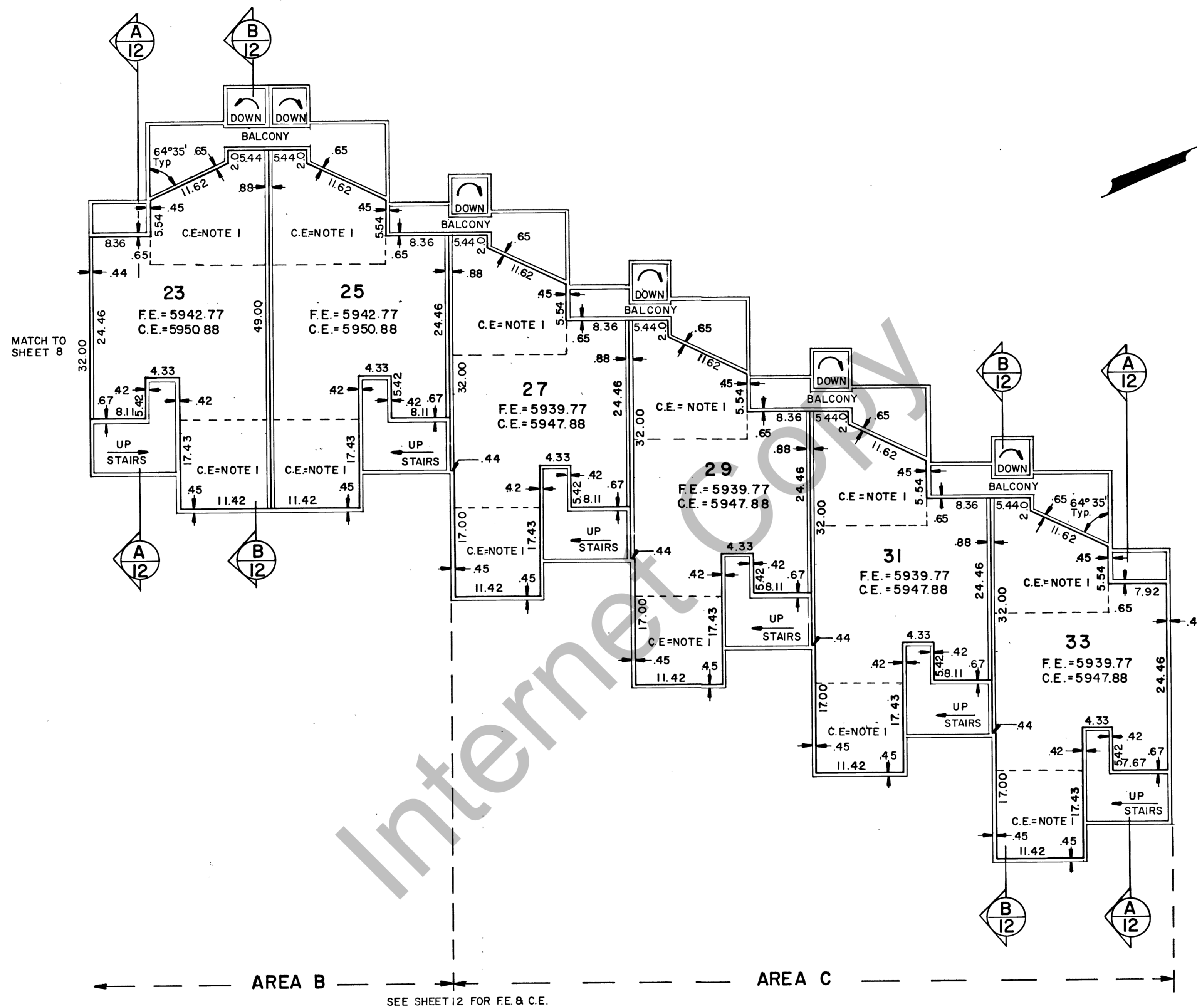
BUILDING B SECOND FLOOR PLAN SCALE: 1" = 10'
