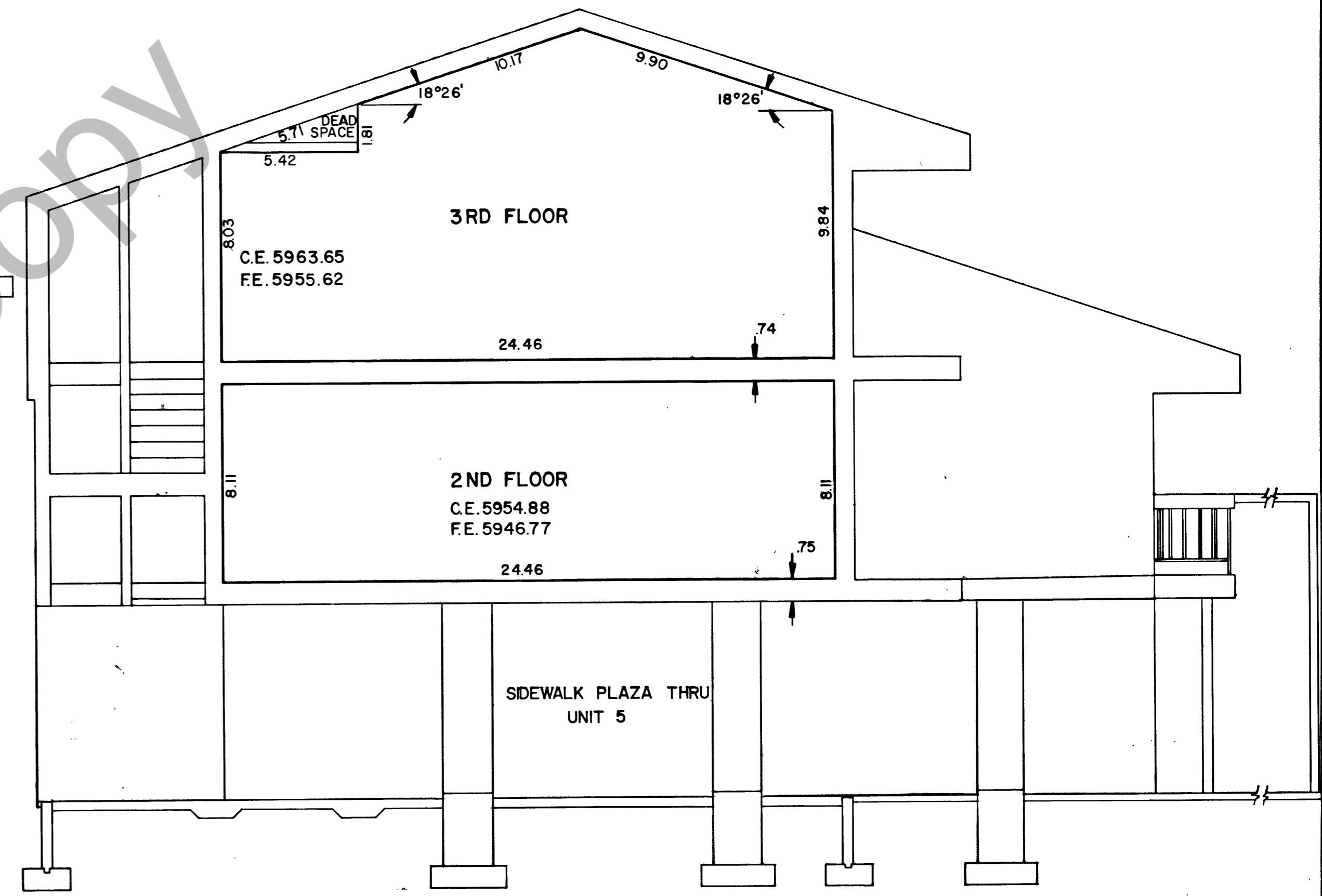
BUILDING A SECTION (C) 5 SCALE: 1" = 4'
