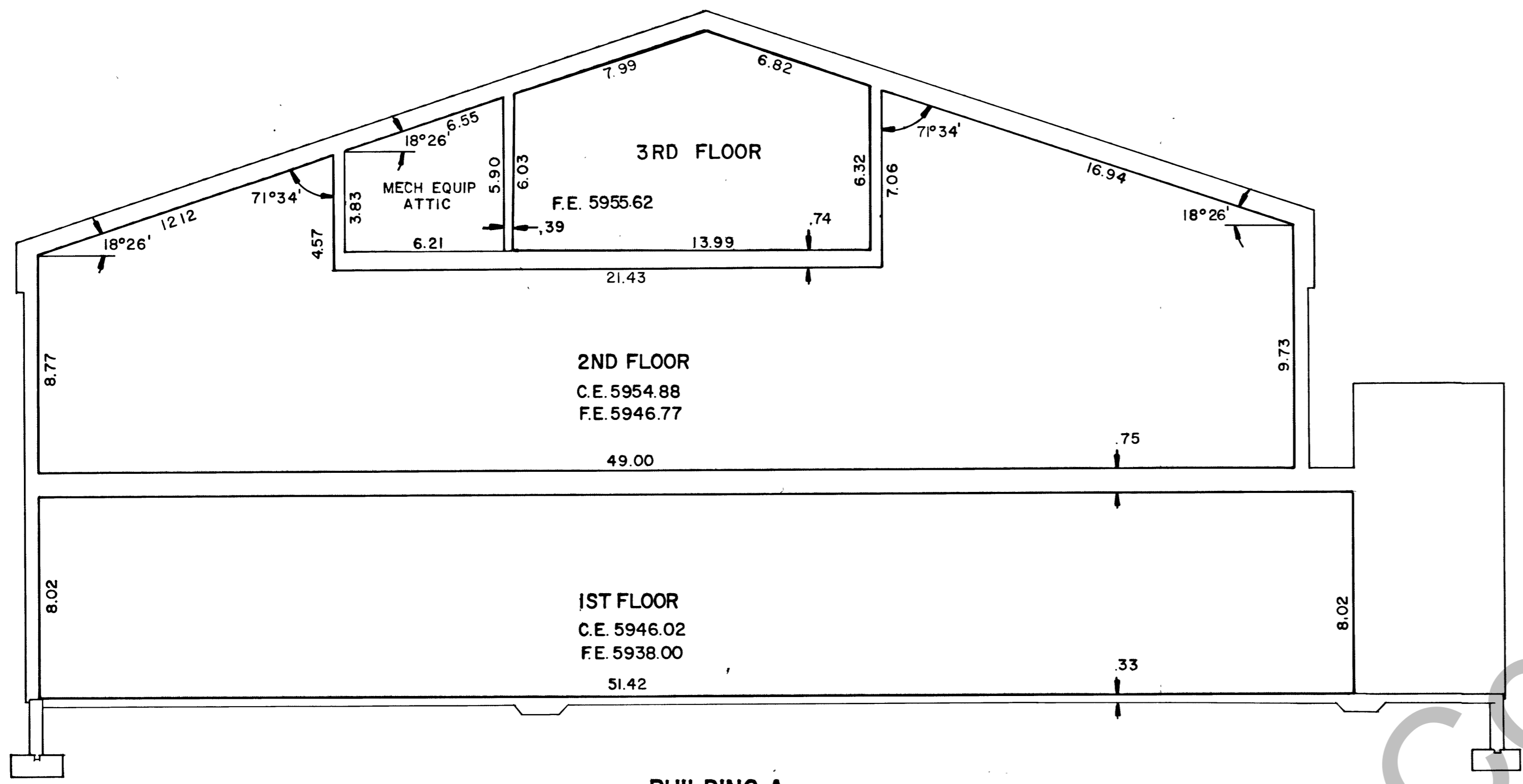
BUILDING A SECTION (B) 5 SCALE: 1" = 4'
