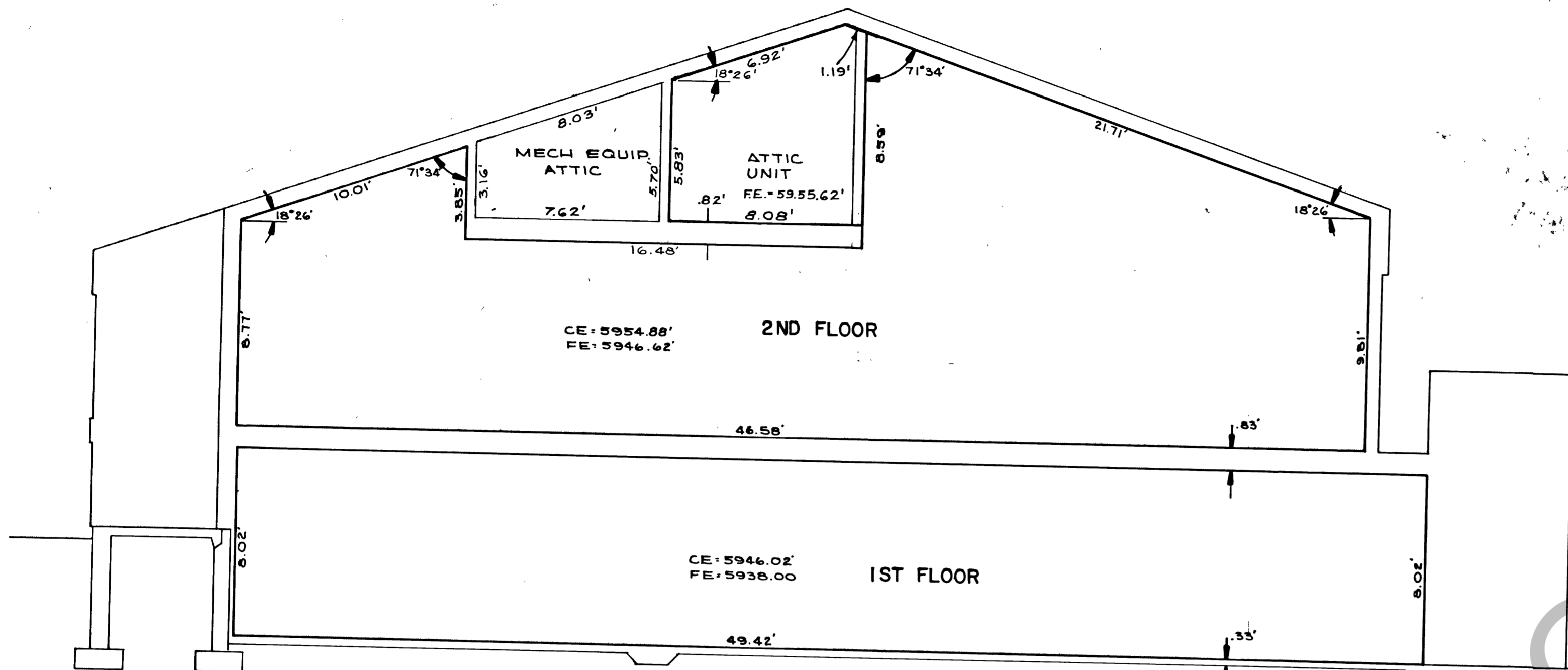
BUILDING B SECTION 10 SCALE: 1" = 4'
