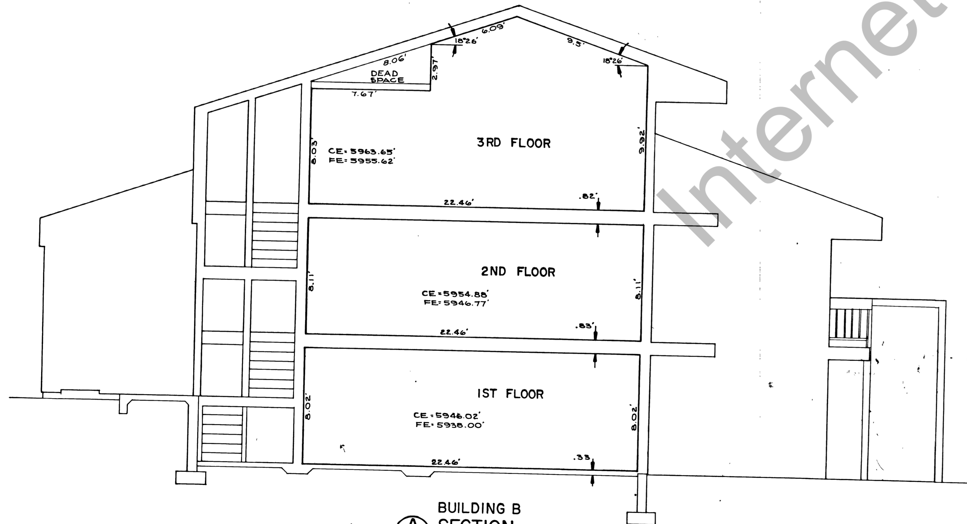
BUILDING B SECTION 10 SCALE: 1" = 4'
