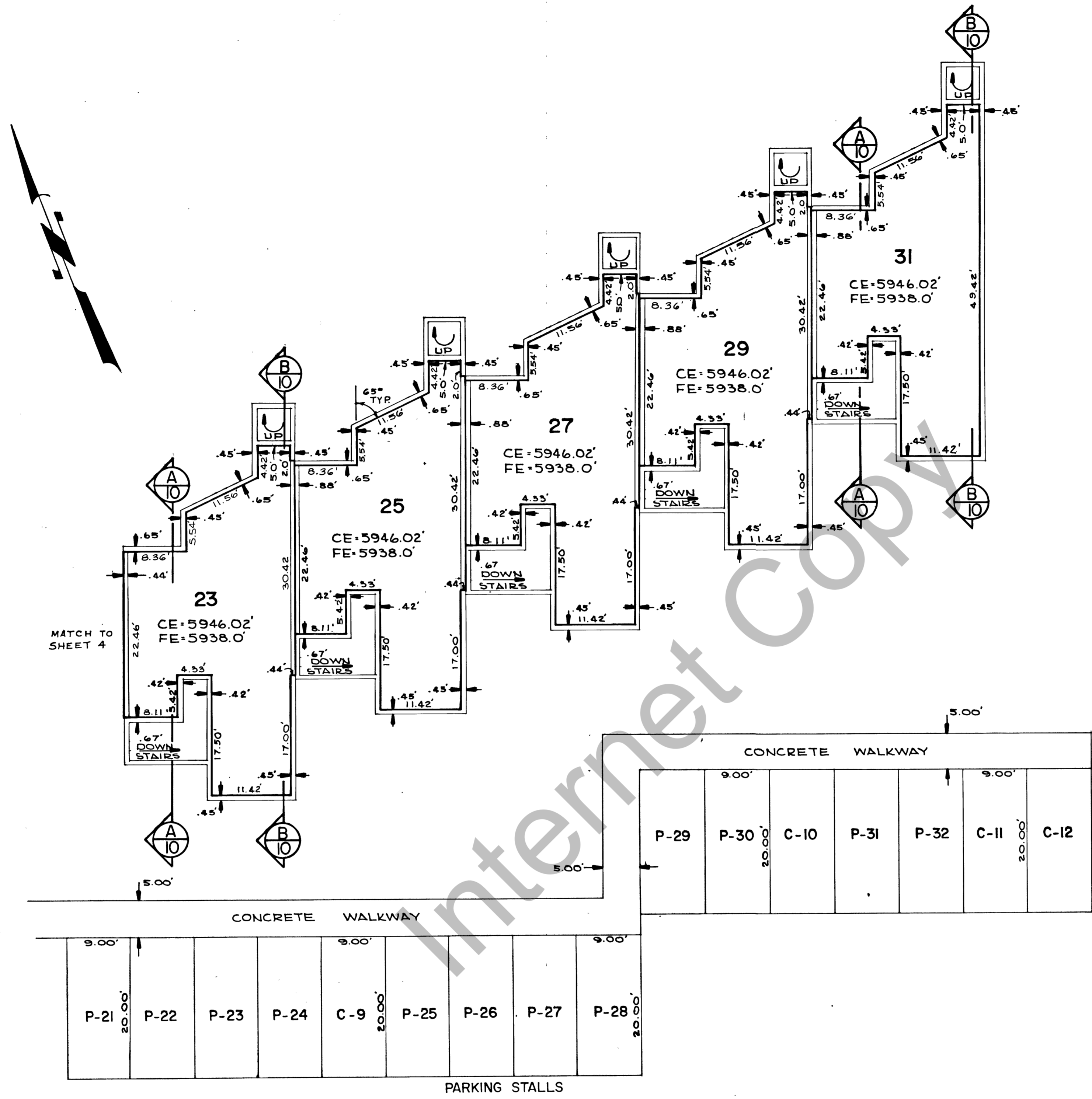
BUILDING B FIRST FLOOR PLAN SCALE: 1" = 10'
